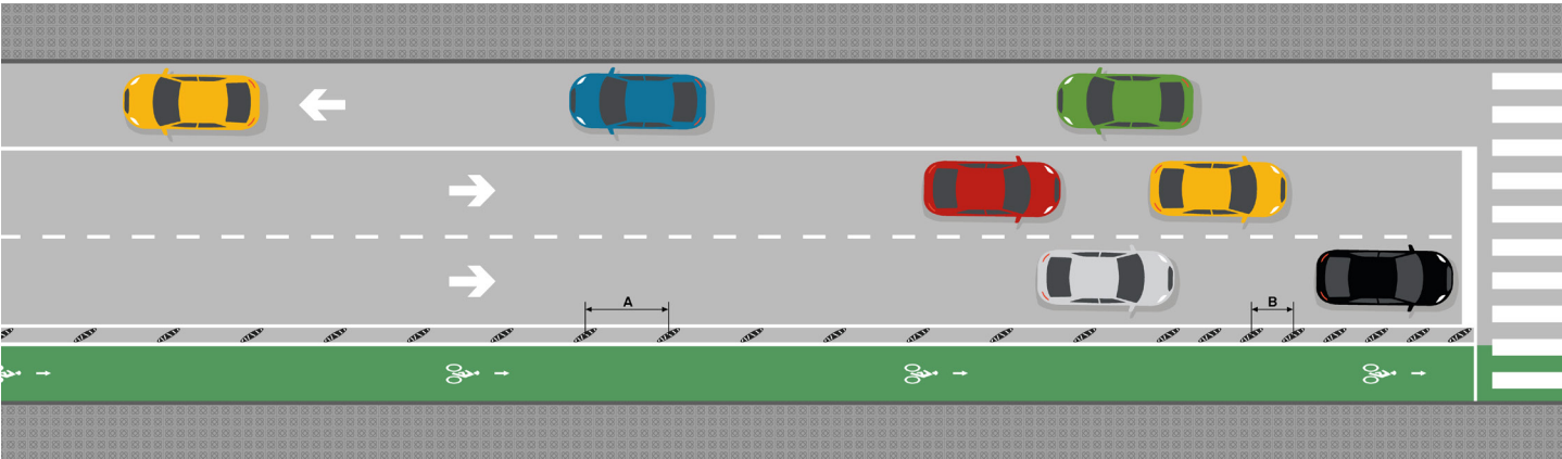
OBLIQUE CONFIGURATION A: 2600 mm (middle of the road). B: 1300 mm (near the intersection).
