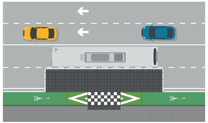
BIKE LANE BOARDER WITH ACCESS BRIDGE 12 m BUS (12,87 m x 4,4 m).
